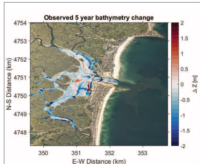
Figure 33-7. Observed bathymetric change from 2011 to 2016.
