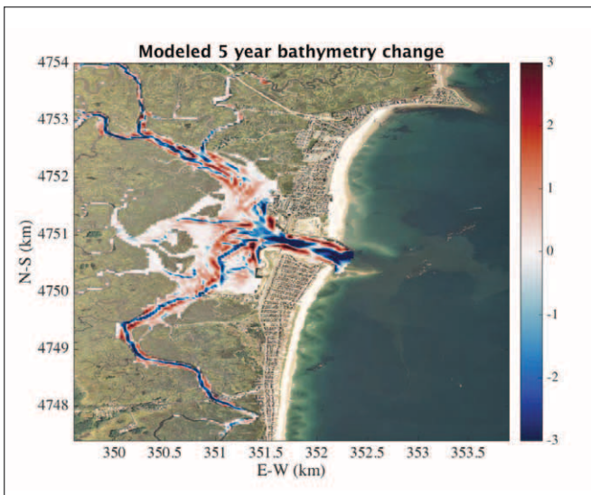
Figure 33-6. Bathymetric difference map from the five-year model run showing distribution of erosion and deposition.
