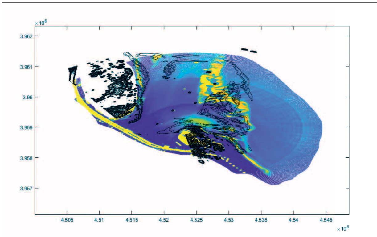
Figure 33-16. Map of Oregon Inlet showing the location of ebb tidal shoal patterns observed in the winter of 2019 (yellow areas) obtained with RIOS radar remote sensing. The black contour lines show the shoal positions observe 2 years previously in 2017 illustrating the dynamic nature of the inlet sedimentary system.
