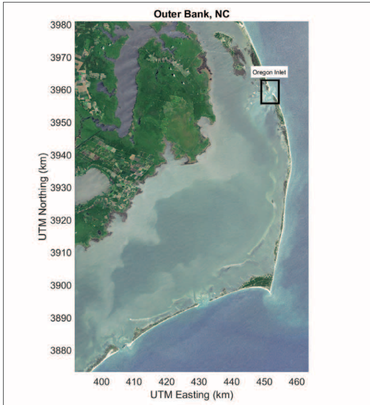
Figure 33-9. Location of Oregon Inlet along the Outer Banks of North Carolina.
