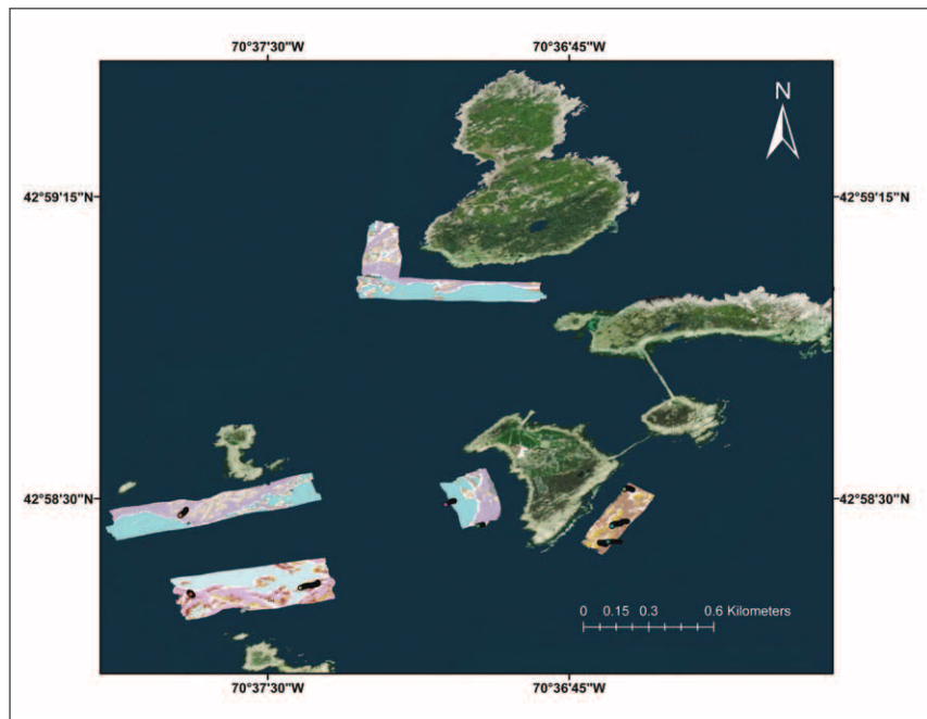
Figure 31-1. Geofoms derived from BRESS observed at six sites at the Isles of Shoals in Maine and New Hampshire. Six landform classes were determined: flat, slope, ridge, valley, shoulder, and footslope.
