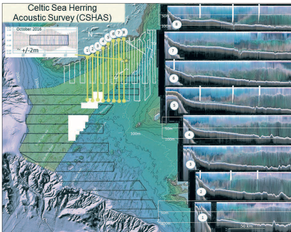
Figure 51-1. Triple Frequency (18-38-120 kHz R-G-B) acoustic imaging of water mass boundaries in the Northern Celtic Sea. Acquired as part of the Annual Herring Acoustic Surveys. Overlain profiles show the temperature structure derived from stationary CTD profiles.
