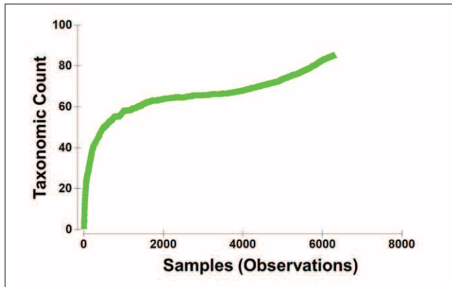
Figure 50-6. Species accumulation curve for taxa observed in the Northeast Canyons. Samples are the number of individuals observed in ROV video footage.
