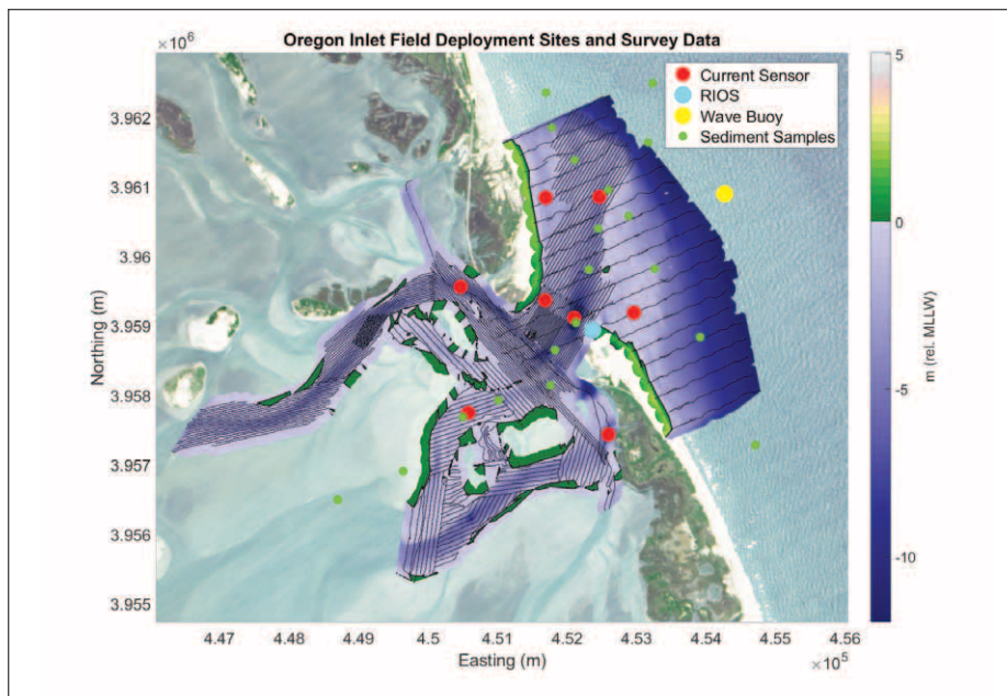
Figure 33-15. Map of Oregon Inlet showing the location of bottom mounted ADCP's (red circles), RIOS radar station (cyan circle), offshore wave buoy and pressure sensor (yellow circle), and sediment grab samples (green dots) deployed for 35 days in the winter of 2019. Single-beam bathymetric survey transect lines are shown with the black lines.
