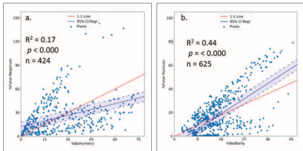
Figure 17-12. Regression lines for the Deeper tile for the percent of errors (FNs or FPs in (a) and (b), respectively) in a pixel relative to its expected percentage ( Bathy or NotBathy for (a) and (b), respectively).
