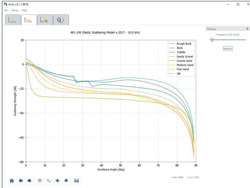
Figure 22-7. Example of model-based angular response curves (at 10 kHz) for several types of sediment, some of them supporting shear waves (i.e., rock).
