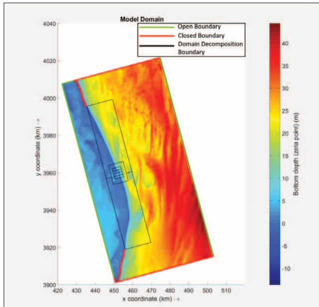
Figure 33-13. Spatial domain showing the nested grids used at Oregon Inlet to model waves, currents, water levels, and sediment transport with Delft3D.
