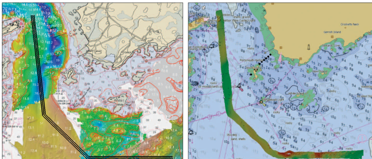
Figure 1-3. Left: Line plan for the 2019 NEWBEX project. Lines have been overlain on top of existing high-resolution bathymetry for the region. Right: Collected bathymetry at 300 kHz.
