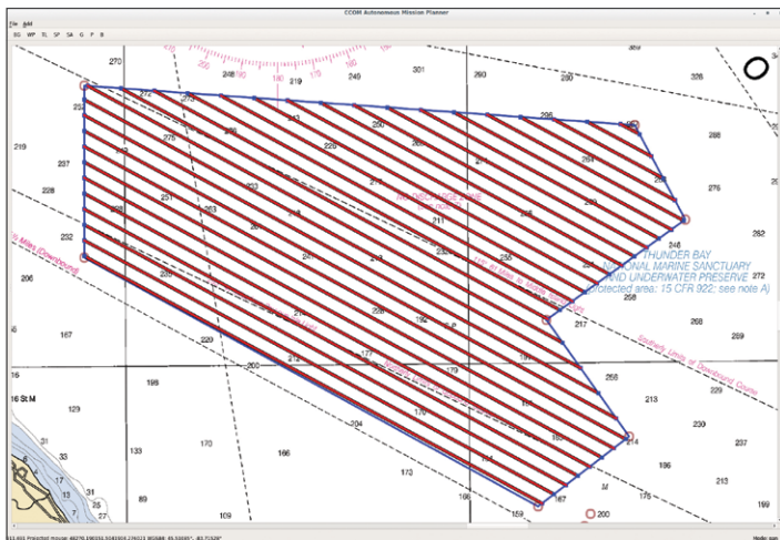
Figure 11-15. The CCOM Autonomous Mission Planner (CAMP) was enhanced with the ability to generate line plans within an arbitrary polygon to adapt to irregularly shaped survey areas.
