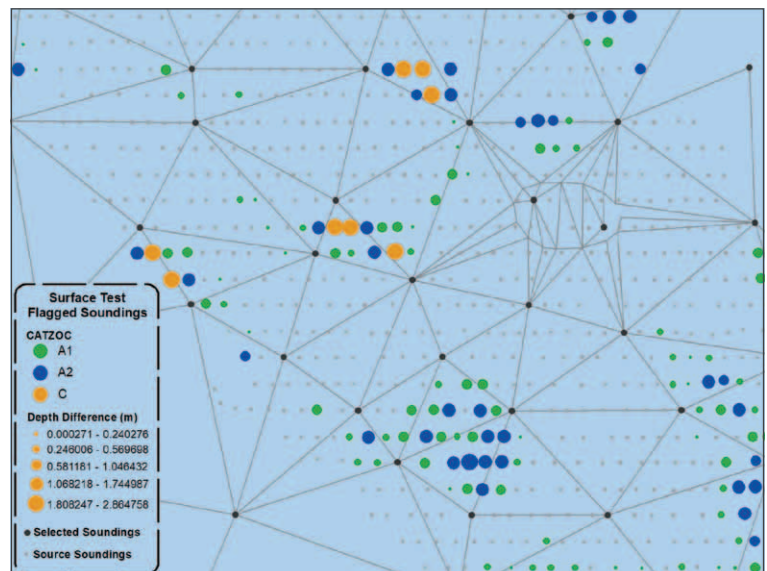
Figure 37-7. Soundings flagged by the nautical surface test tool that is being tested by MCD.
