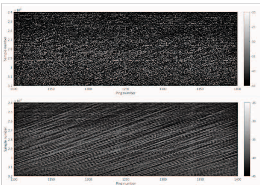
Figure 20-7. A subset of the original match filtered acoustic data (top panel) and the spatially filter dataset (bottom panel).
