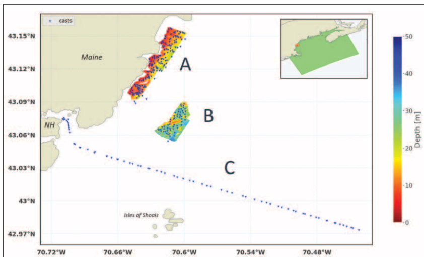
Figure 8-6. Bathymetric coverage completed by the UNH Hydrographic Field Course 2019. The collected casts (in blue) were grouped into three subsets: the “A” and “B” subsets corresponds to the two distinct surveyed areas, the “C” subset was collected during an offshore-sailing transect. The inset shows the locations of the survey area (red-framed yellow rectangle) and the GoMOFS domain (green tilted rectangle) in the Gulf of Maine.
