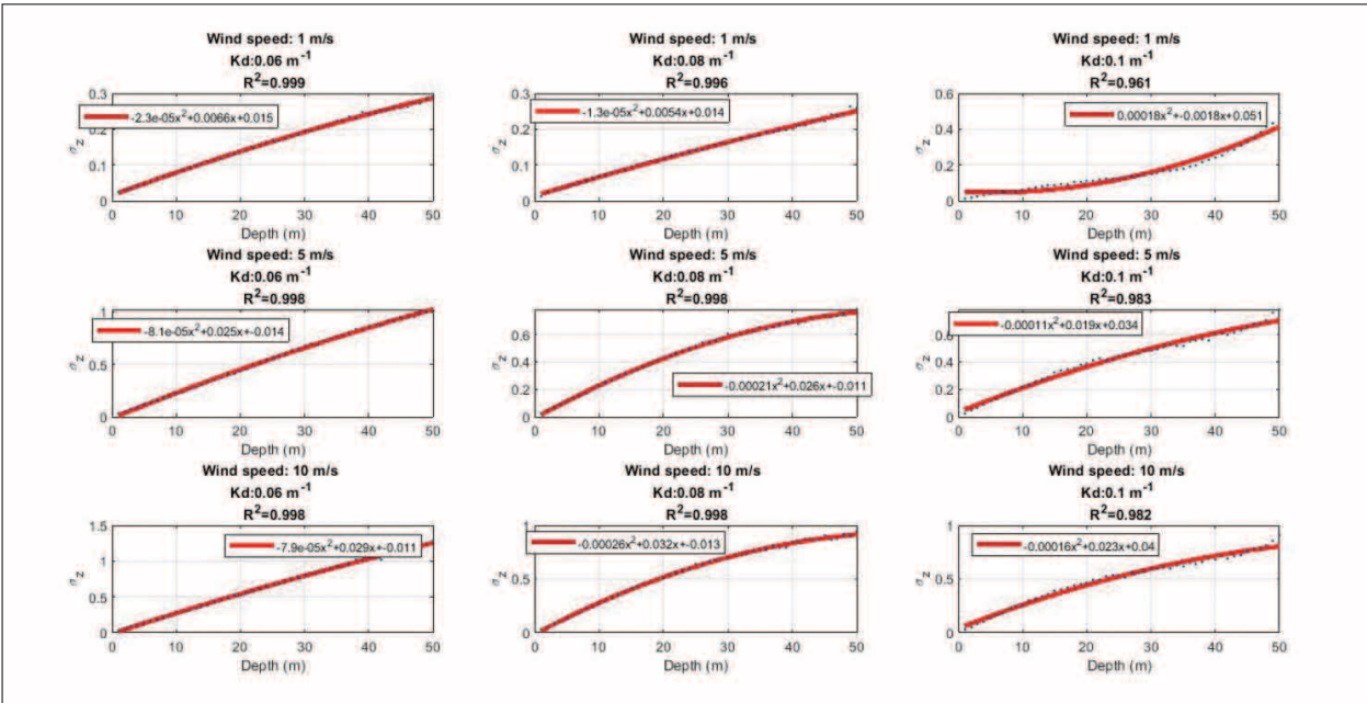
Figure 17-6. A sampling of the simulation results for CZMIL and their polynomial fit: depth vs. \sigma_z for wind speeds of 1, 5, and 10 m/s and Kd of 0.06, 0.08, 0.1 m -1 .
