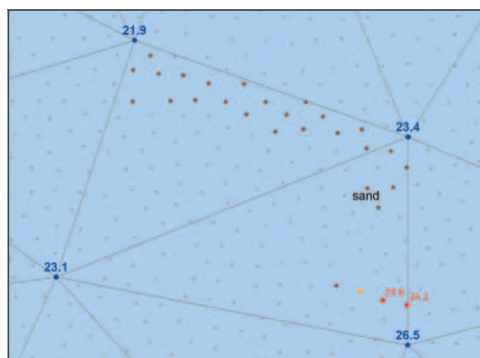
Figure 37-5. Example of the proposal nautical surface test. The NST identified multiple locations where the expected depth is deeper than the source information. Those in dark grey fall within ZOC A1 limits and may be ignored, that in orange falls within A2, and, worse, those in red would fall within ZOC C.
