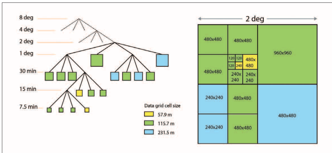
Figure 45-5. An example of a quadtree metagrid hierarchy. To the left, as a standard tree diagram. To the right, the same structure is shown as a map. Different resolutions are color coded.
