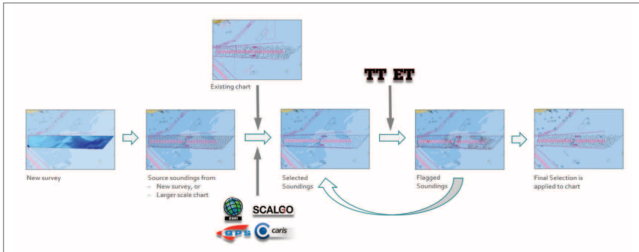
Figure 37-1. Process for turning source information into charted soundings.
