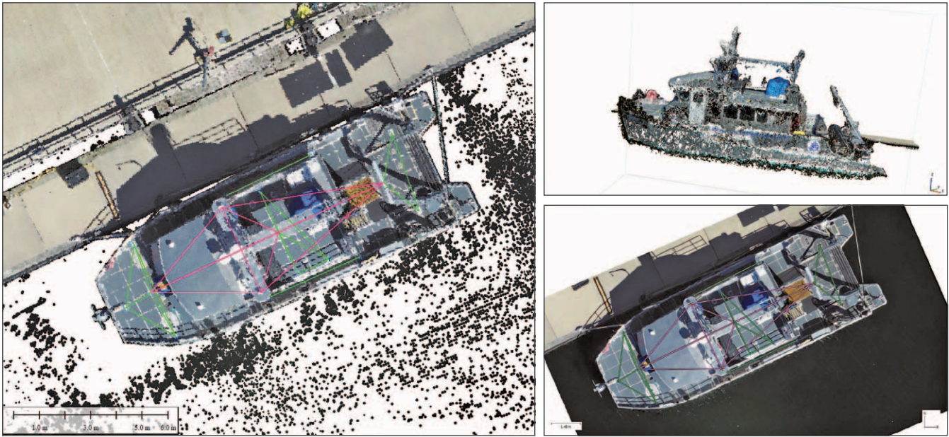
Figure ES-14. Left: Point cloud for the R/V Gulf Surveyor constructed using aerial LiDAR from a DJI Matrice UAV at multiple altitudes. Note the lines joining survey monuments (purple) and Secchi targets (green), which are measured in the point cloud to assess the technique. Upper-right: Point cloud created using Structure from Motion (SfM) techniques from drone photogrammetry. Lower-right: Orthomosaic of the R/V Gulf Surveyor corresponding to the point cloud on left. Note the lines joining survey monuments (purple) and Secchi targets (green), which are measured in the orthomosaic to assess the technique.
