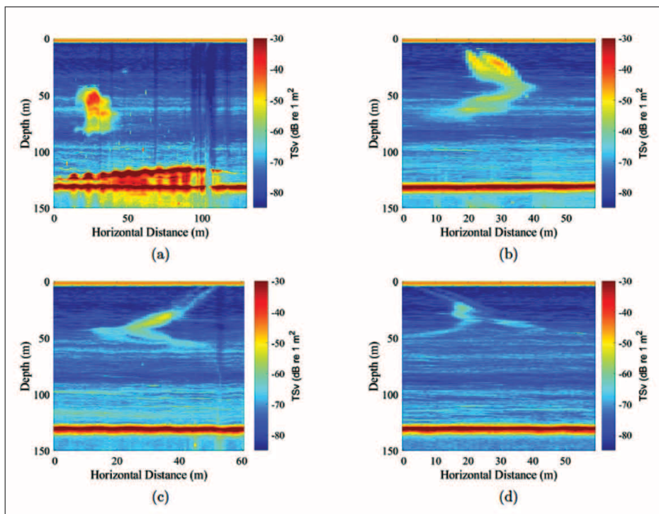
Figure 20-1. (Loranger's Figure 4.3, PhD dissertation). Echograms for cross sectional passes downstream of the Taylor seep origin. (a) is the echogram closes to the origin (58 m), followed by (b) (115 m) then (c) (187 m) and (d) (235 m).
