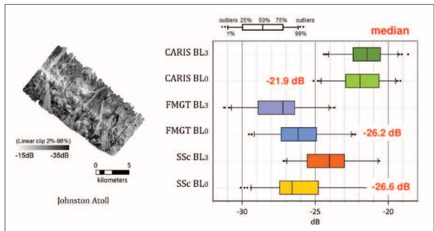
Figure 22-1. Results of a preliminary study that compares the mosaics created using different popular applications and options. The survey data were collected with a Kongsberg EM 302. BL0 represents the backscatter values retrieved from the raw data file; BL3 is the value obtained after all the corrections have been applied (before mosaicking). Intermediate processing stages have provided insights into differences between software outputs. In particular, the differences in BL0 values were not anticipated.
