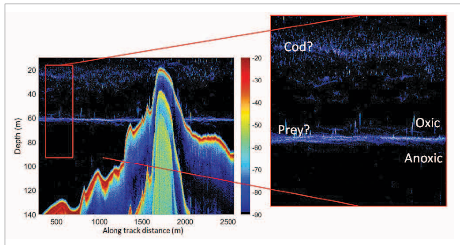
Figure 51-5. Preliminary EK80 echogram from EL18-B5. The scattering layer at the top of the hypoxic region is visible at approximately 60 meters depth.
