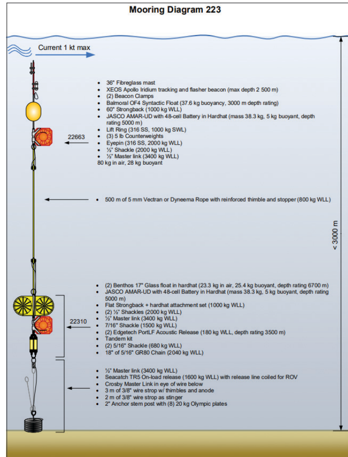
Figure 54-2. Notional mooring diagram provided by JASCO and deployed at both AUTEC in December 2018 and at SCORE in January 2019.
