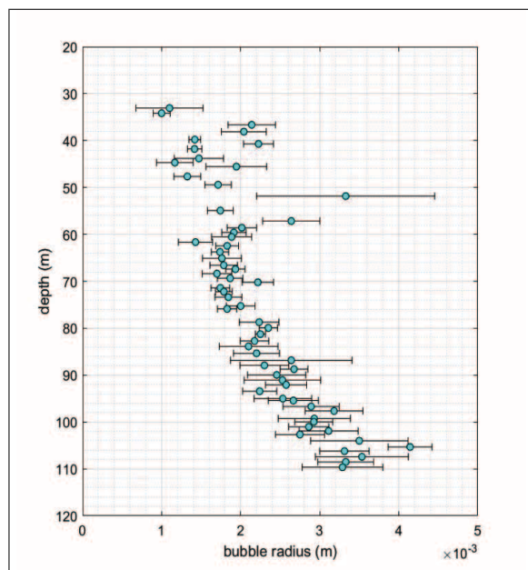
Figure 19-4. Derived bubble radii from a single ES200 pass.
