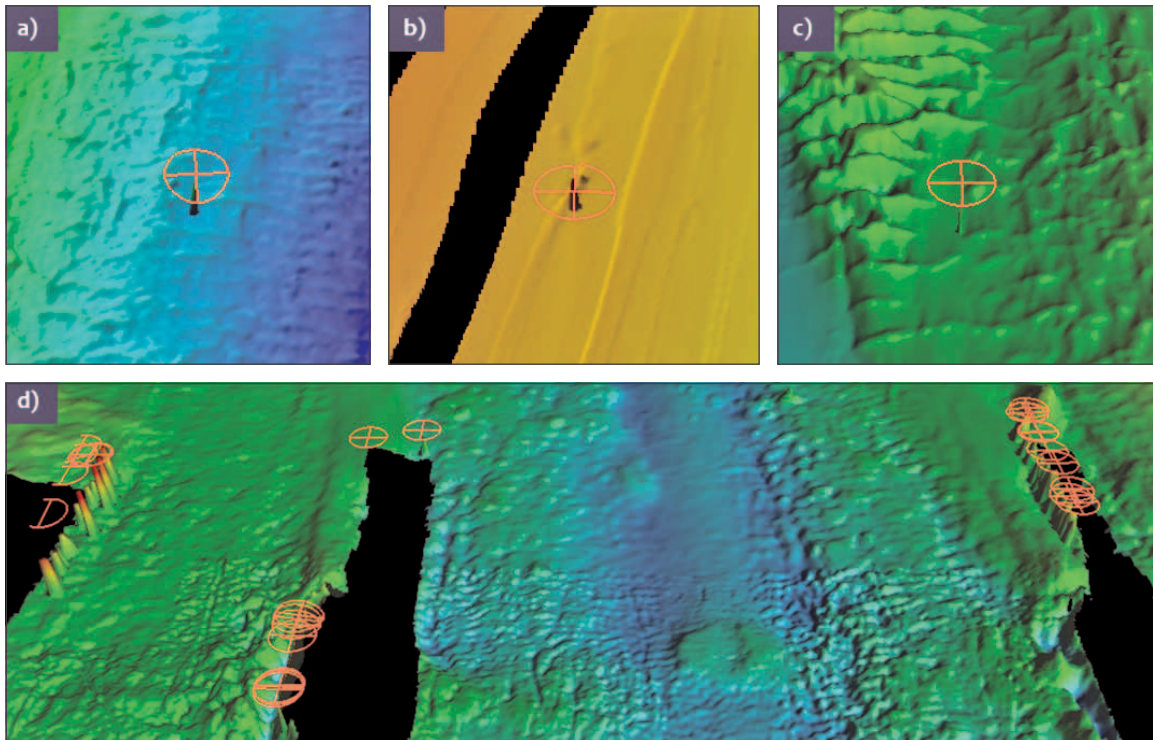
Figure 15-3. Improvements in the Find Fliers sub-algorithm. The upper panes ('a', 'b', and 'c') show examples of identified fliers using the 'traditional' set of bathymetric anomaly detection algorithms. Recently adopted technologies in the NOAA OCS workflow have generated a new type of fliers that required the introduction of dedicated 'noisy edges' algorithm (examples of detected fliers are shown in pane 'd').
