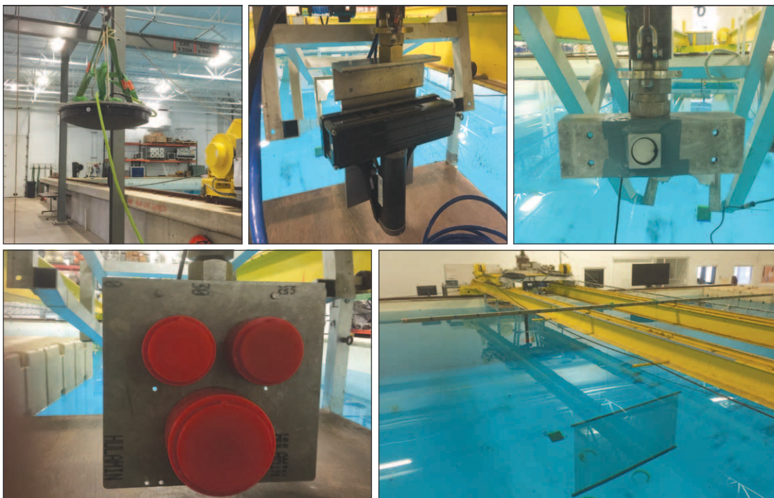
Figure 1-1. Tests in the acoustic tank in 2019. Top Left: MSI LF CBT; Top Center: Reson T50-P; Top Right: Custom-built transducer; Bottom Left: Simrad split-beam echosounders; Bottom Right: Standard chain target.
