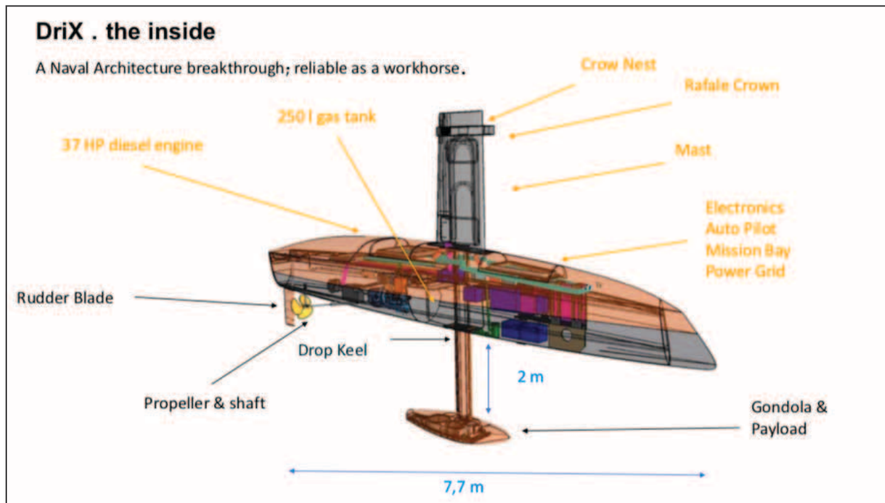
Figure I-19. Schematic of the iXblue DriX autonomous surface vehicle.
