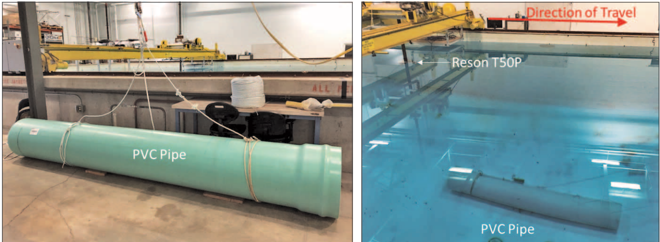
Figure 14-2. PVC pipe deployed in the tank and used for testing multidetect algorithms in the Chase Lab engineering tank.
