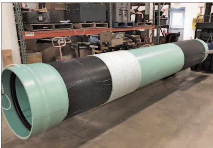
Figure 14-4. The pipe with a 'roughened' surface consisting of antiskid tape and a wrap of potwarp (left image), and the deployment of the pipe at sea using the R/V Gulf Surveyor .
