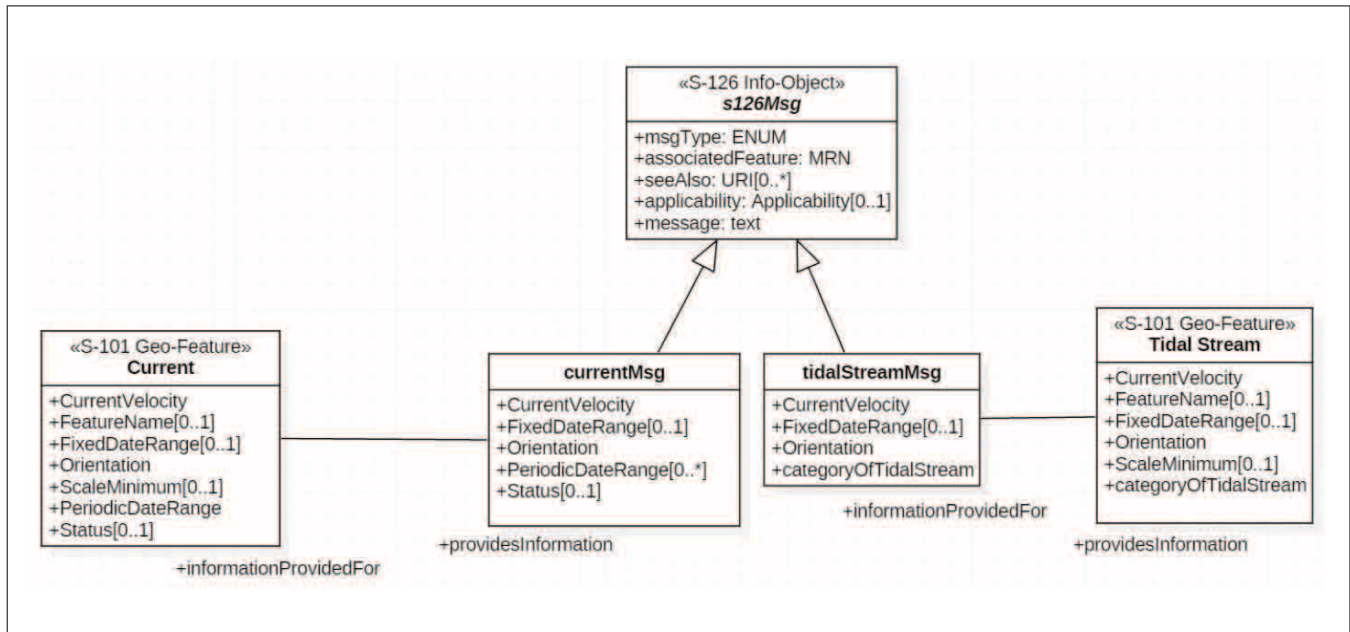
Figure 43-2. Prototype data model designed to support textual data relating to the physical environment presented to NIPWG6.
