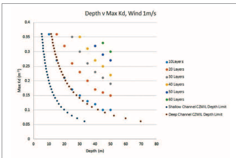
Figure 17-5. The maximum K_d that can be used to compute uncertainty at a depth, by number of scattering layers for a wind speed of 1m/s. The deep and shallow channel depth limits described by the specification sheet are also plotted. The deep channel limit is very closely aligned to the simulation limits with 10 layers.
