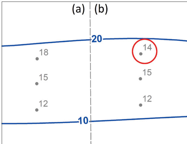
Figure 37-2. Source sounding (14m) that deviates significantly from the expected depth, but which the triangle and edge tests fail to identify due to their intrinsic limitation.
