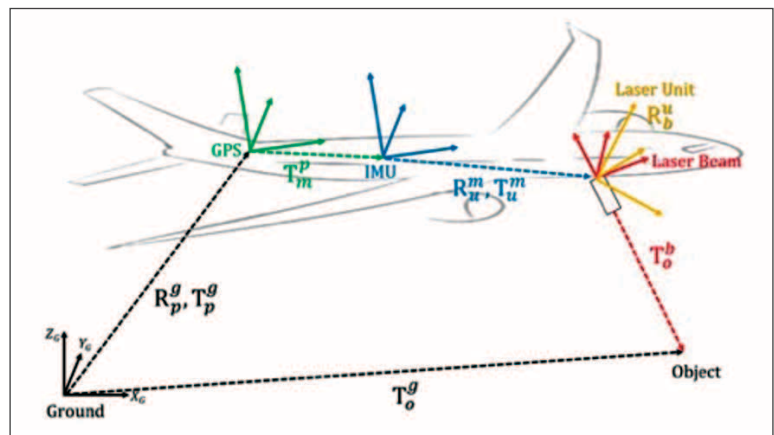
Figure 17-3. Improved geo-location model for cBLUE, which includes boresight calibration misalignments. These are typically small but can be significant in some cases.
