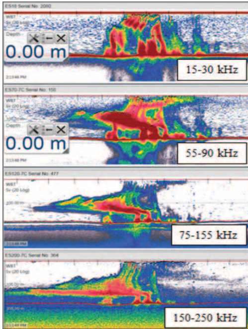
Figure 19-5. Multi-frequency response of the FOI-2 system.
