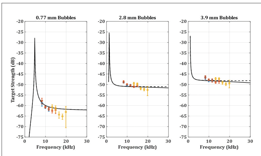
Figure 20-3. Target strength measurements from bubbles, such as those shown in Figure 20-2, in comparison with standardly used TS models. The data points and the vertical error bars represent the mean and the mean plus/minus the standard deviation of TS estimates obtained from a vertically-oriented echo sounder operating with LFM pulses of 8-13 kHz (blue), 8.05-16.1 kHz (red), and 12-20 kHz (yellow).
