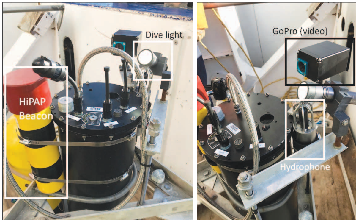
Figure 19-1. The bubble generator and auxiliary equipment employed during bubble generator deployment operations: positioning beacon, video camera/dive light, and hydrophone.
