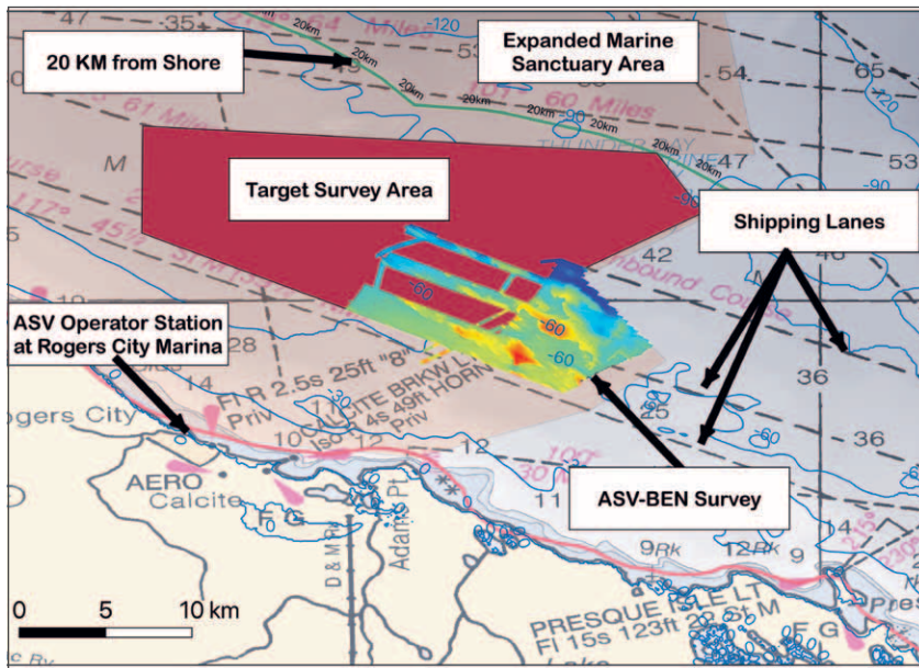
Figure 11-1. ASV-mapped area from the Thunder Bay National Marine Sanctuary Mapping Expedition. The ASV was operated from shore at Rogers City Marina, surveying between shipping lanes more than 10-25 km distant (data credit: OET/UNH-CCOM).
