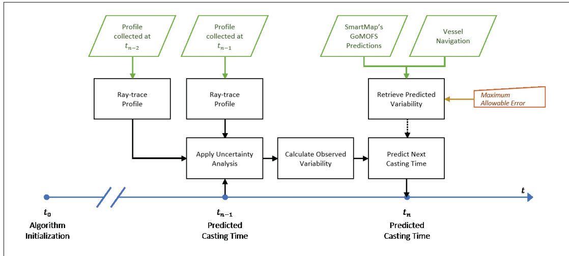
Figure 8-11. The ForeCast algorithm. The flowchart shows, in black, the main steps of the with a dashed connector when optional (i.e., the predictive component based on SmartMap’s GoMOFS maps). The inputs are represented in green, the user parameter in orange, and the timeline in blue.
