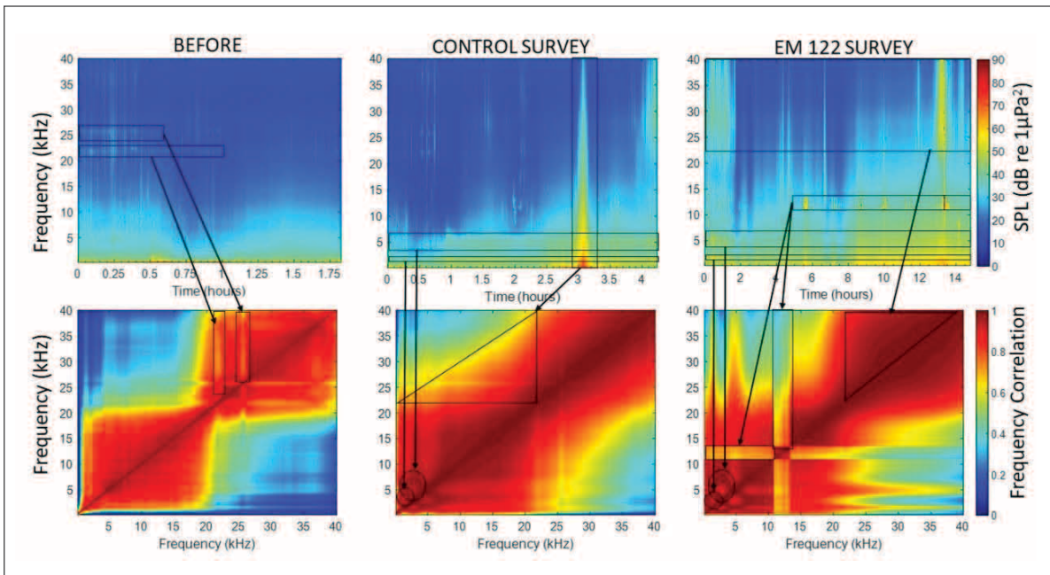
Figure 56-7. Frequency correlation plots for the three time periods on hydrophone 404 (bottom row) in comparison to respective spectrograms (top row). Black boxes and arrows indicate how the content of the two plots relate.
