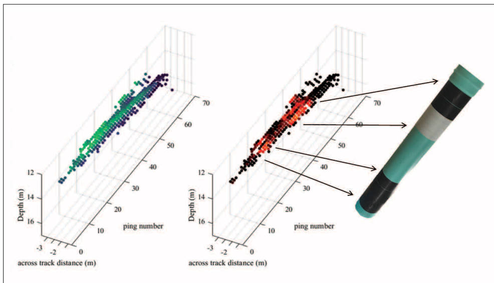
Figure 14-6. Pipe soundings extracted from our multi-detect soundings showing both depth (left) and backscatter (right). Hotter colors are shallower (left) and stronger backscatter (right).
