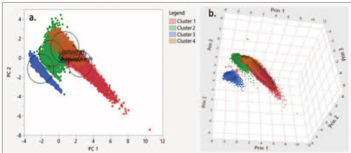
Figure 17-13. Example of normal mixtures clustering for the Deeper tile using four classes.
