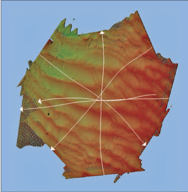
Figure 1-4. The bathymetry of a star pattern with the track lines overlain. The backscatter data collected from these patterns will be used to determine if there is an azimuthal dependence to the collection of backscatter.
