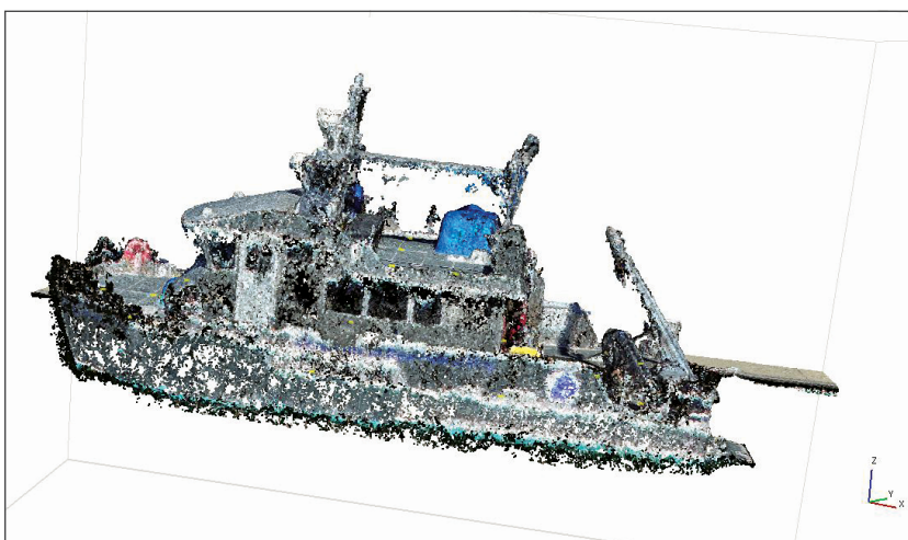
Figure 12-4. Point-cloud for the R/V Gulf Surveyor constructed using Structure from Motion (SfM) techniques applied to the drone photogrammetry survey at an altitude of 31m.
