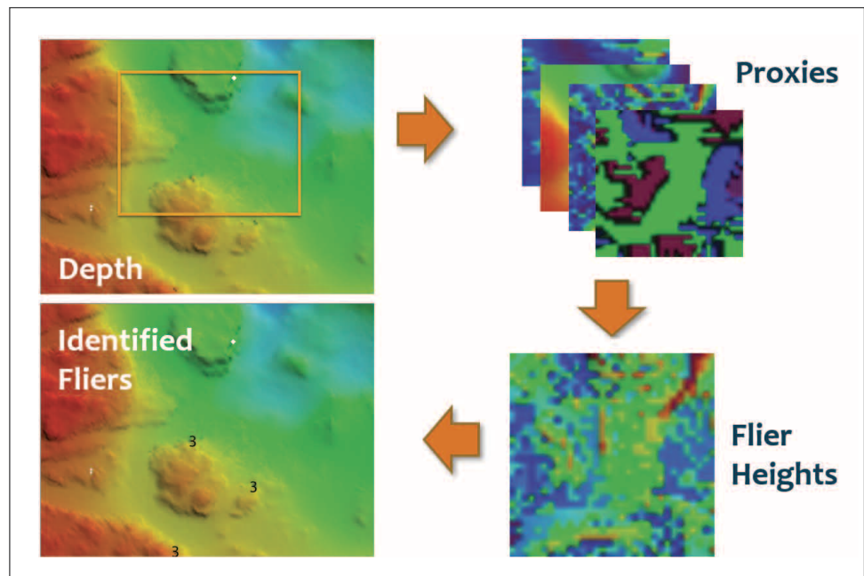
Figure 15-2. Structure of the Anomaly Detector algorithm. This calculates localized flier heights using grid-derived proxies, potentially resulting in fewer false positives and missed fliers.
