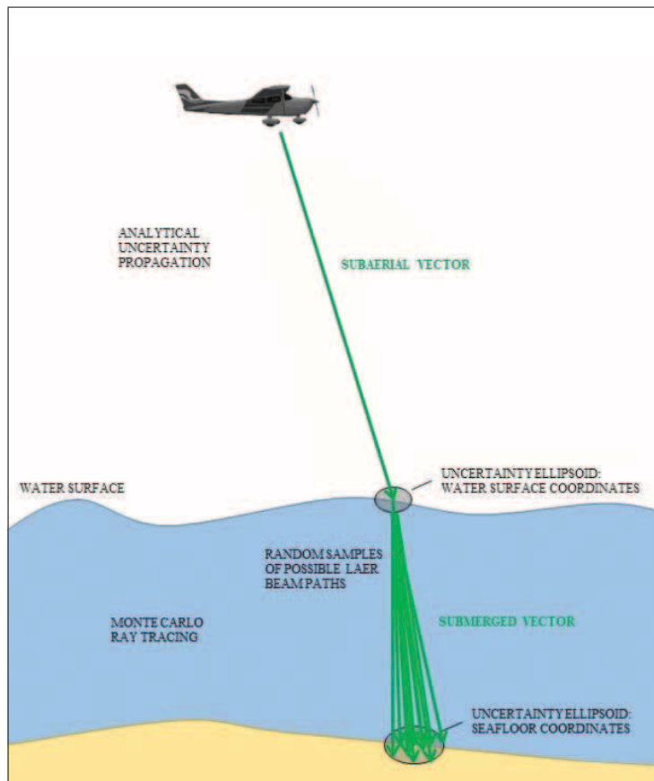
Figure 17-1. Decomposition of the two main uncertainty factors for topobathy lidar systems: the sub-aerial (lidar to water) and sub-aqueous (water to seafloor) components.
