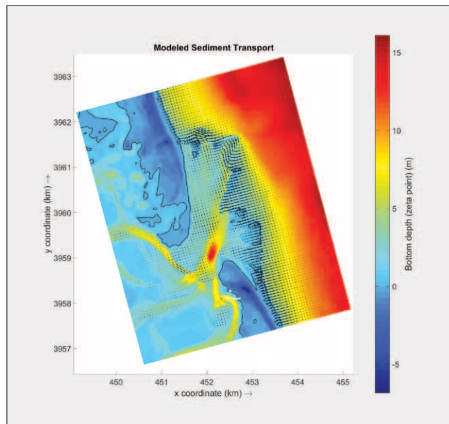
Figure 33-14. Preliminary model run showing the modeled currents and resulting bathymetry over a 30-day period at Oregon Inlet with Delft3D.
