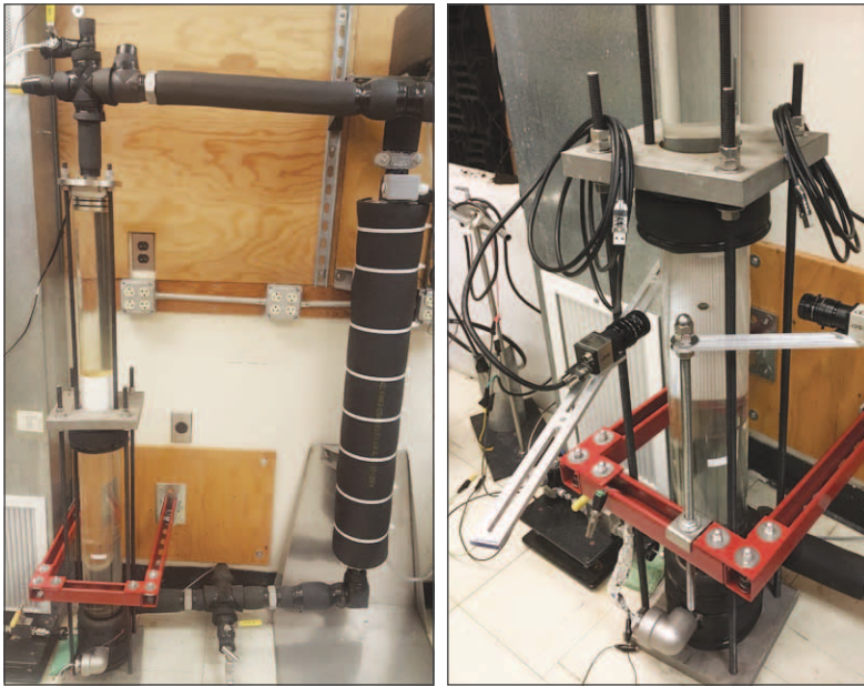
Figure 20-4. An image of the USGS flow loop device, used to examine hydrate-coated Xenon bubbles.
