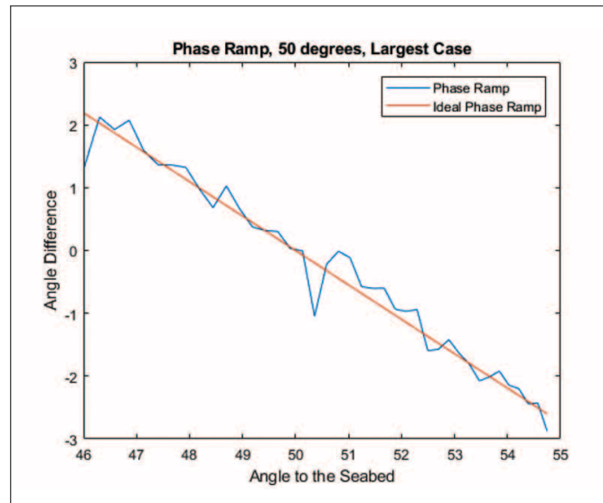
Figure 3-5. The phase-difference observed at the receive pair shown in Figure 3-3 for the case where only the main beam is considered in the seabed response (left), and the case where the full simulation including main beam and sidelobes is considered (right). The blue line is the observed (simulated) phase ramp, and the red line is the ideal analytical solution based on the geometry of the seabed and the receiver pair. Note that 50° corresponds to the angle to the (flat) seabed which is perpendicular to the receiver baseline.
