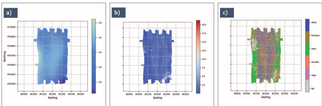
Figure 18-4. Experimental algorithm to automatically determine a spatially-adaptive flatness parameter. Pane 'a' shows the input bathymetry (values in meters). In pane 'b', the adaptive flatness threshold values (in degrees) are visualized, obtained by retrieving the 25th percentile among all the valid slopes surrounding each node, then applying Gaussian smoothing. Pane 'c' shows the resulting landforms based on a six-type classification table.
