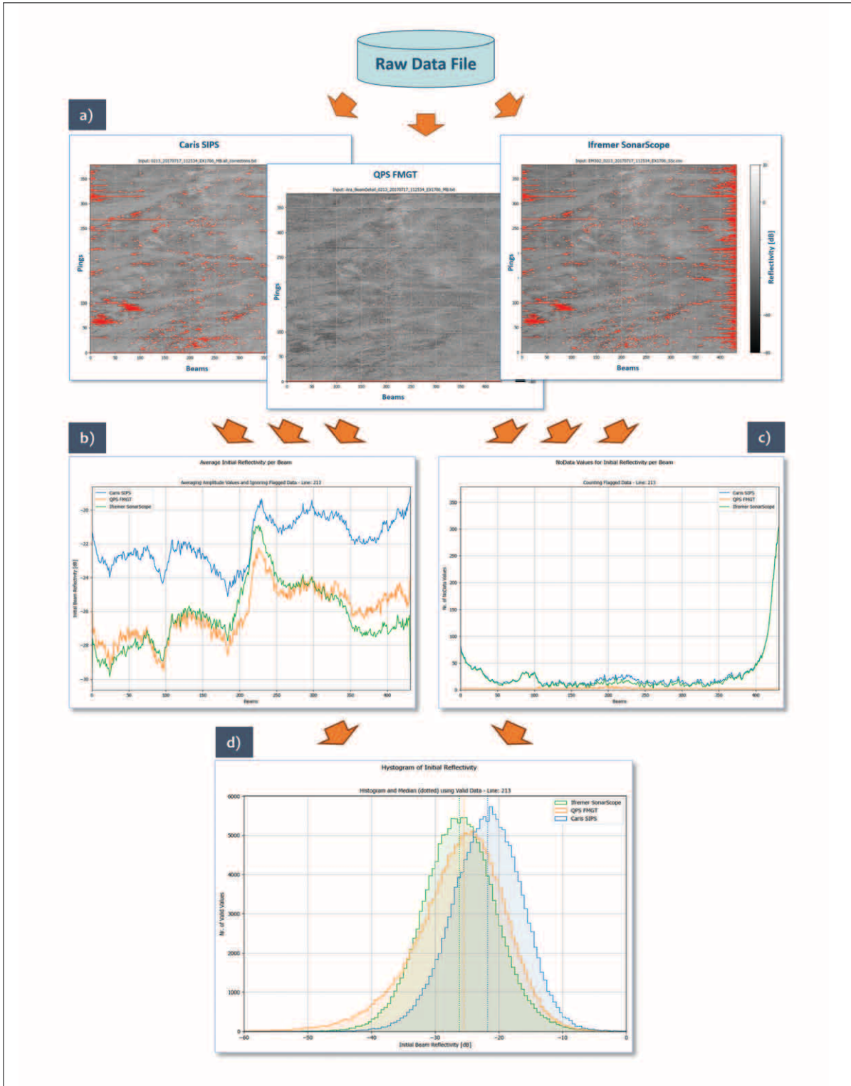
Figure 22-2. Pane 'a' shows the initial reflectivity values calculated by three software packages (and retrieved from the same raw data file) in a ping-beam geometry. Pane 'b' plots, for each package, the average value per beam across the whole survey line. Similarly, pane 'c' displays the number of no data values per beam. Finally, pane 'd' compares the resulting histograms for the three software packages highlighting how the resulting statistical characteristics starts to diverge since the very first processing step.
