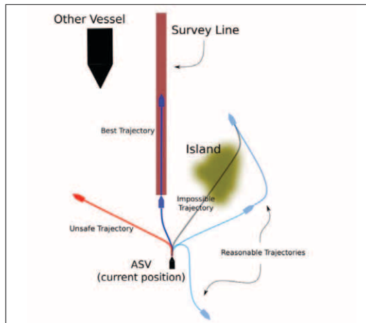
Figure 11-14. Conceptual drawing of the Real-time Motion Planning for Path Coverage algorithm, in which safe paths are sought that prioritize the survey mission.
