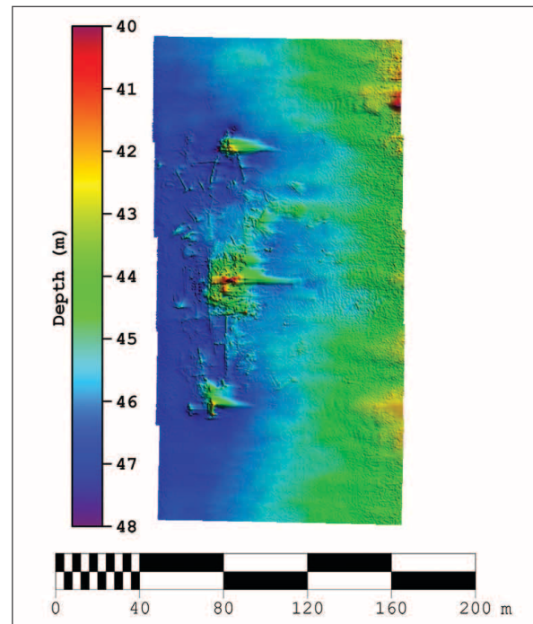
Figure 4-2. Bathymetric map of a shipwreck site off of Virginia using the KATFISH towed SAS system.
