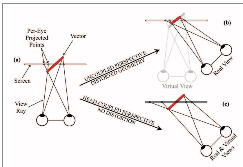
Figure 45-1. Correct stereoscopic viewing on a desktop monitor requires the user’s view and the virtual projection to match (a), (c); otherwise the vector glyph length (red) will appear distorted (b) because the visual system receives incorrect information about the 3D scene.
