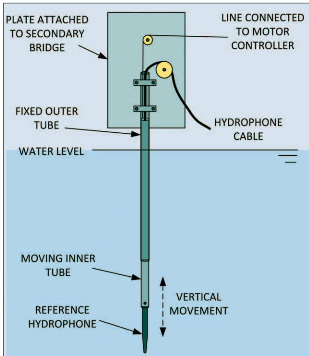
Figure 1-2. Vertical position control of reference hydrophone.
