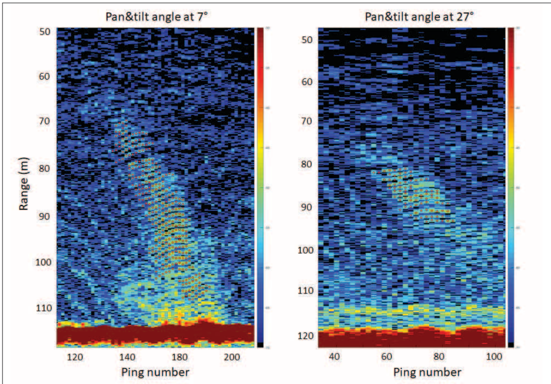
Figure 19-3. Examples of processes ES200 data from the pan&tilt system at 7 degrees (left) and 27 degrees (right).
