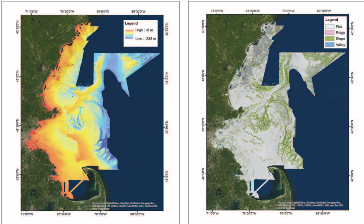
Figure 21-3. Western Gulf of Maine Bathymetry synthesis composed of MBES surveys gridded at 16 m (left panel). BRESS landform analysis of the bathymetry (right panel). Figures 21-4 and 21-5 are enlargements of the BRESS landform map.
