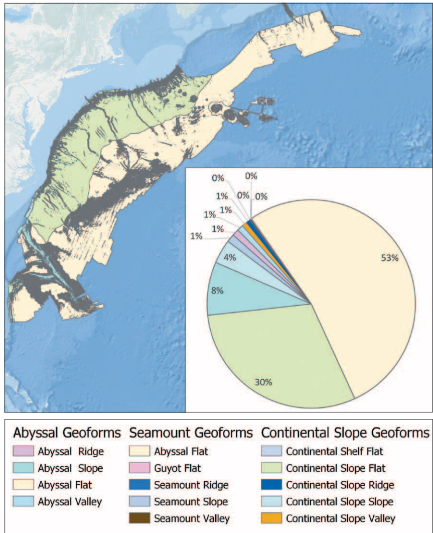
Figure 50-1. CMECS geomorphology classifications for the entire Atlantic Margin region in the study.
