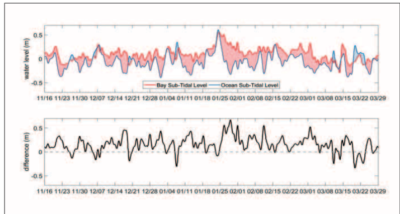
Figure 33-11. Differences in sub-tidal water level variations across the inlet create a dynamic residual pressure gradient which primarily forces a sound to ocean flow.
