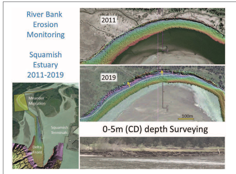
Figure 30-2. Scour Erosion of Salt Marshes through Meander Migration.
