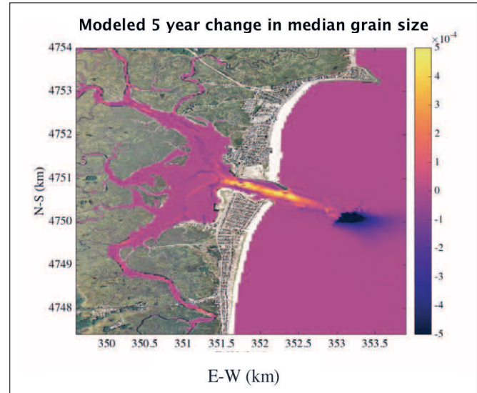
Figure 33-5. Change in median grain size distribution after the five-year model run.
