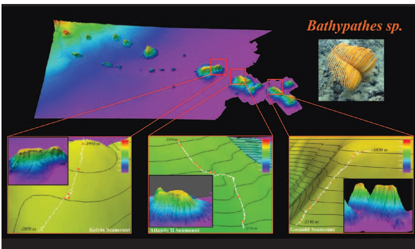
Figure 50-5. ROV tracks showing the wide distribution of black coral observed on Kelvin, Atlantis II, and Gosnold Seamounts.
