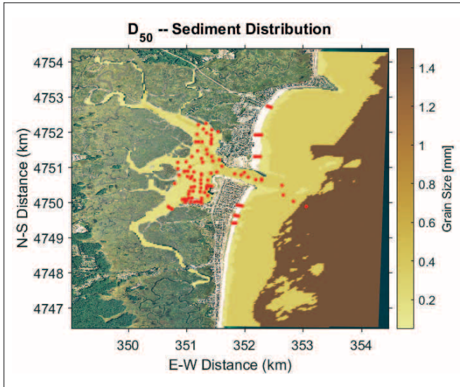
Figure 33-4. Hampton/Seabrook Harbor showing the location of sediment samples (red dots) obtained from 2000-2015 and used to develop the sediment size distribution for the model grid.
