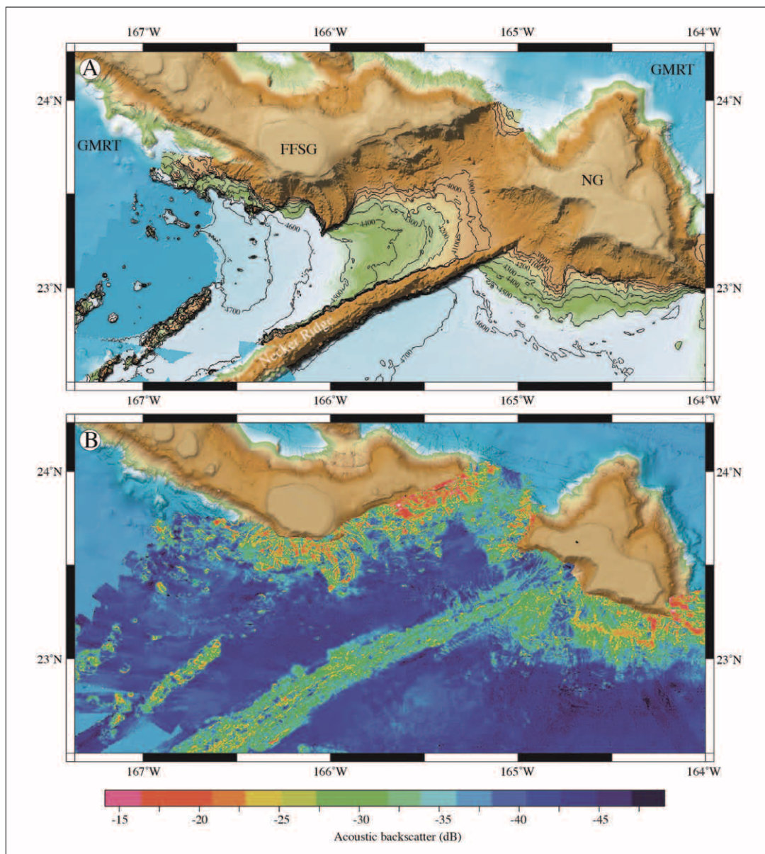
Figure 48-3. Map view of MBES bathymetry of archipelagic aprons on the south flanks and adjacent abyssal seafloor of French Frigate Shoals (FFS) and Necker Island (NI) on the Hawaiian Ridge.
