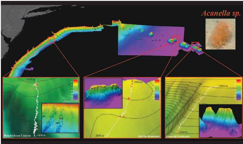
Figure 50-3. ROV tracks showing the distribution of bamboo corals collected in Hendrickson Canyon, Kelvin and Gosnold Seamounts.
