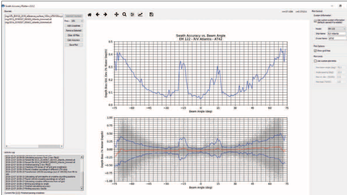
Figure 8-14. Swath accuracy analysis GUI under development in a joint MAC-NOAA project, showing mean biases (red) and standard deviations (blue) of deep-water MBES soundings relative to a bathymetric reference surface. Test data are binned in 1° increments across the swath and may be plotted in meters or as a percentage of water depth. The GUI provides additional plotting control and will support archive of test data to track system behavior over time, compare performance to other installations, and examine the effects of varying operational settings (e.g., runtime parameters, vessel noise, and sea state).
