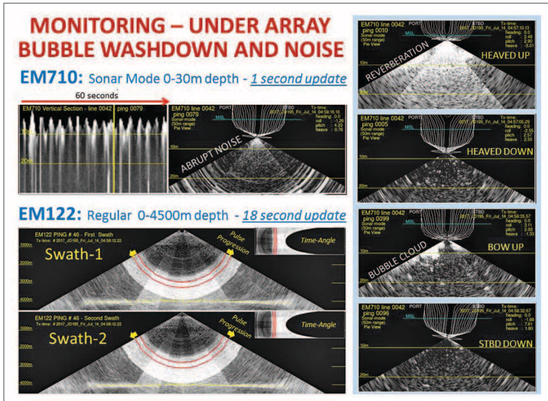
Figure 7-4. Simultaneous monitoring of near-array scattering and its effect on multi-second, deep-water multibeam performance. Top-left shows 60 seconds curtain of volume scattering within 30 m of the surface, together with instantaneous across track view of the scattering field. Bottom-left shows an 18-second ping cycle of an EM122, highlighting the 1-second period during which the near array image above was collected. Right shows stills of an animation showing the second-by-second evolution of the scattering field immediately under the hull during a single EM122 ping cycle.
