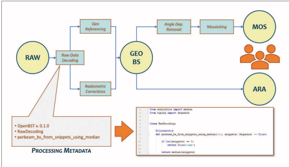
Figure 22-3. The backscatter users usually work with the backscatter mosaics and/or the angular response curves. These products are at the end of the processing workflow (i.e., after raw data decoding, geo-referencing, application of radiometric corrections), thus far from the initial data input. As such, it is difficult to identify where divergence occurs, thus the software processing workflow appears like a black box to the final users. For each processing step, OpenBST adds a processing metadata entry providing information about which library release and which method was adopted. This solution uniquely identifies the processing operation.
