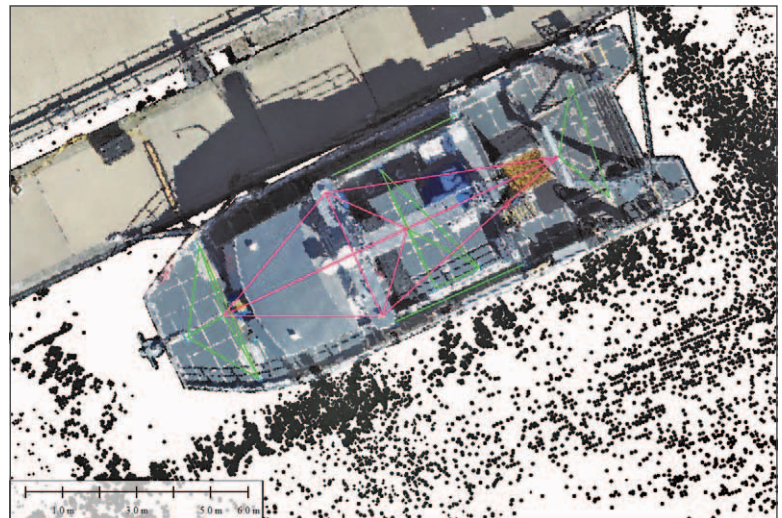
Figure 12-3. Point-cloud for the R/V Gulf Surveyor constructed using aerial LiDAR from a DJI Matrice UAV at multiple altitudes. Note the lines joining survey monuments (purple) and Secchi targets (green), which are measured in the point cloud to assess the technique.
