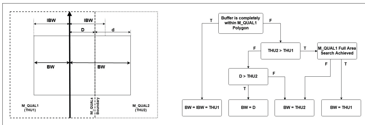
Figure 37-18. Preliminary decision tree for the width of the zone on both sides of the plotted course.
