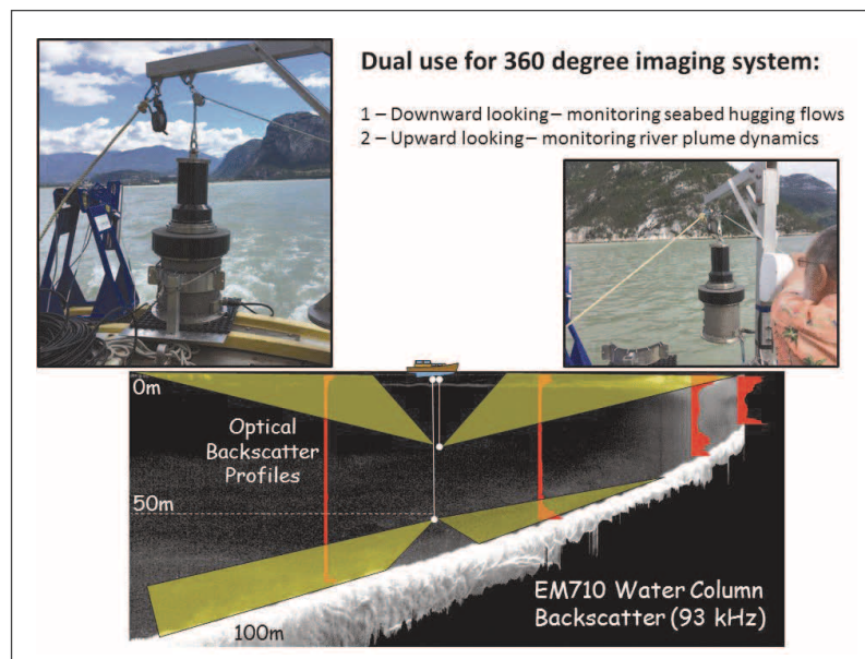
Figure 30-3. Showing the DDS-9001 sonar head on board CSL Heron and the geometry of deployment.
