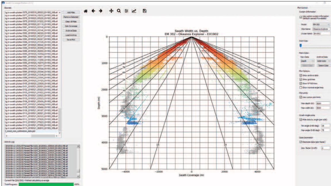
Figure 8-13. Swath coverage plotter GUI under development in a joint MAC-NOAA project, showing recent (EX1902, colored by depth) and archive (EX1802, gray) soundings for comparison of coverage achieved by the NOAA Ship Okeanos Explorer . The user has improved control over plotting and archiving data for comparison of a system to itself and others throughout its service life. Development is ongoing for this and other GUIs to simplify routine performance monitoring for multibeam operators throughout the UNOLS, NOAA, and academic fleets.
