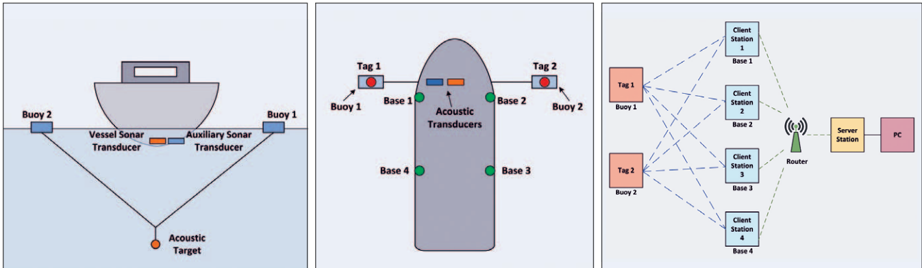
Figure 1-5. Left: Target positioning mechanism using remote-controlled buoys; Center: Location system setup on vessel; Right: Real time location of tagged buoys using radio transceivers diagram.
