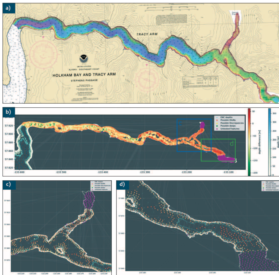
Figure 15-5. Field example of the Chart Comparison tool. Pane a: bathymetric model generated using the data collected by from NOAA survey H13071. NOAA raster nautical chart (Holkham Bay and Tracy Arm) is shown in the background. Pane b shows the results of the Chart Comparison tool using survey H13006's soundings compared to the US4AK35M ENC. Axes in geographical WGS84 coordinates. The areas in panes c and d were selected to illustrate the large detected chart discrepancies.
