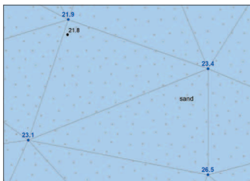
Figure 37-4. Example of conventional selected sounding testing. With only the 21.8m source sounding flagged through the triangle and edge tests, one may conclude that the area enclosed by the two triangles meets the safety constraint.
