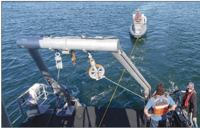
Figure I-12. Towing the DriX Autonomous Surface Vessel and launcher behind the R/V Gulf Surveyor .
