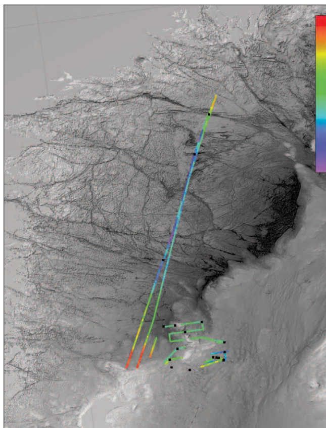
Figure 51-8. Overview of the oxygen minimum depth across the entire survey area, as computed from the acoustic peak reflection coefficient.
