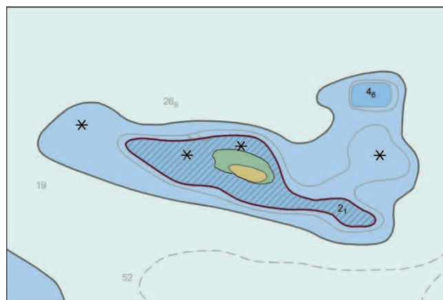
Figure 37-10. Depth area encoded in different units than the Adjoining depth area and the delimited depth curve (i.e., fathoms vs meters).
