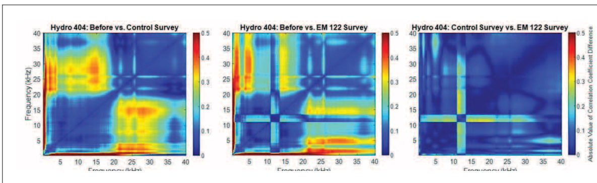
Figure 56-8. Frequency correlation difference plots, comparing each pair of time periods on hydrophone 404.
