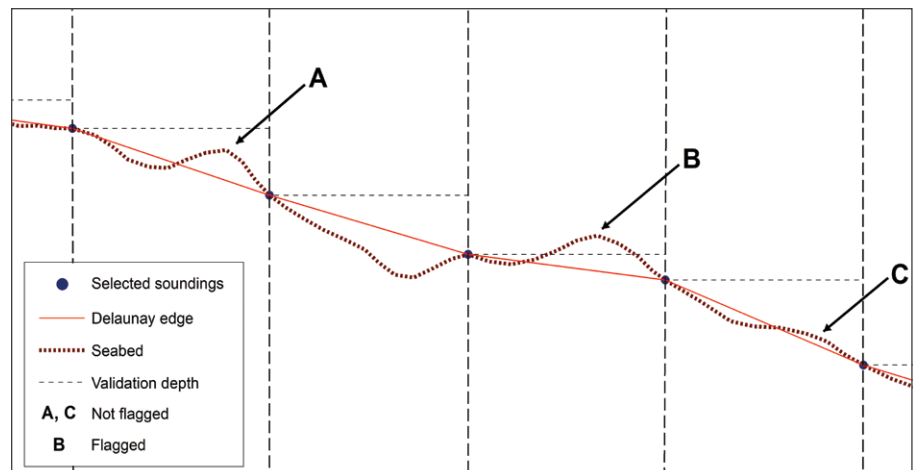
Figure 37-3. A profile view of the seabed, the selected soundings, and the Delaunay faces showing why the two tests fail to identify eminences that deviate significantly from the expected depth on chart.
