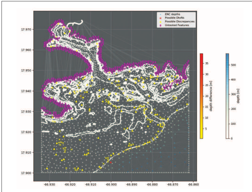
Figure 15-8. Results from the combined workflow obtained using the Soundings Selection and the Chart Comparison tools. The survey's selected soundings, obtained from the survey PR-1401's bathymetric grid, are compared to the US5PR63M ENC. Axes in geographical WGS84 coordinates.
