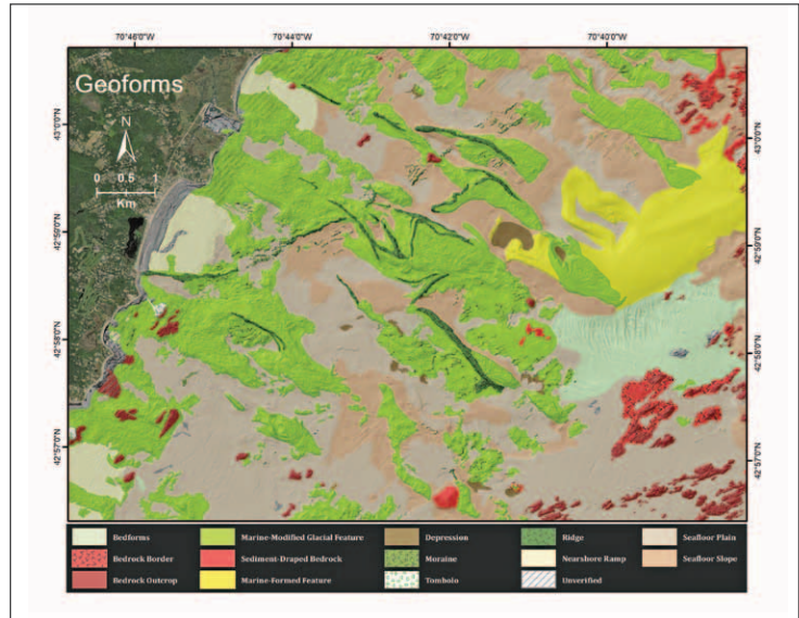
Figure 21-1. Surficial geology map of the nearshore continental shelf landward of the Isles of Shoals, NH showing the major geoforms. The seafloor is characterized by eroded glacial features (leaving behind megaclast deposits) and seafloor plains. The BRESS landform analysis of the same area is shown in Figure 21-2. Marine-modified glacial features are shown in green, marine formed features in yellow, seafloor plains in beige, depressions in brown, bedrock outcrops in red, nearshore ramps in ivory, and bedform fields in mint green. Dark grey areas are unmapped.
