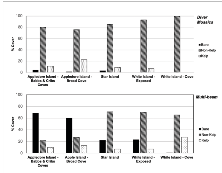
Figure 31-4. Comparison of ground-truth photomosaics (A) and acoustic derived (B) percent cover of kelp, non-kelp and bare substrate (see text for further explanation).
