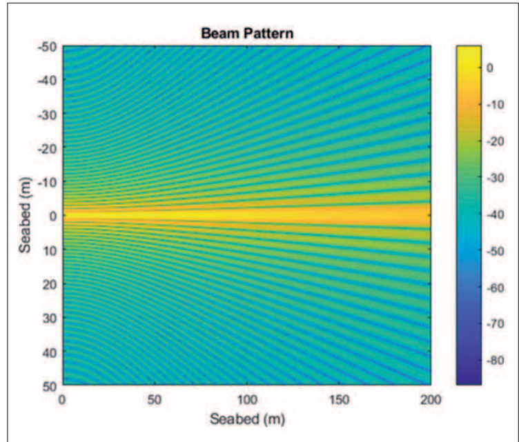
Figure 3-4. The transmit beam pattern imposed on the simulated seabed.
