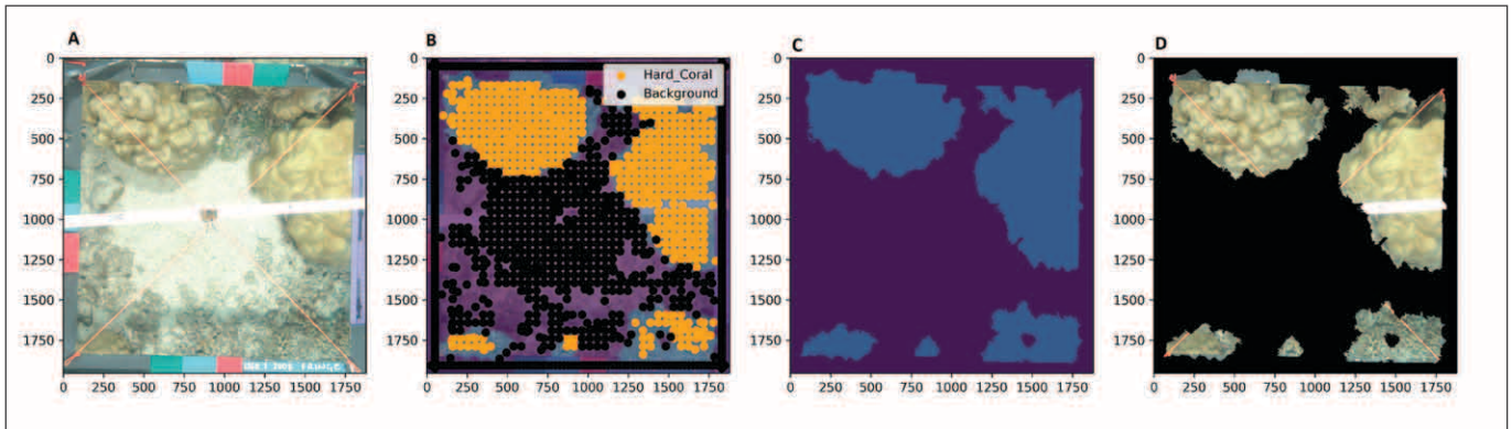
Figure 31-6. Process of generating masks for each class category and its use as training data for the deep semantic segmentation algorithm: (A) Sample image from the MLC (2000x2000 pixels) dataset (B) Image with more labelled points by trained artificial intelligence that act as autonomous annotator, (C) Groupings of pixels belonging to the same class category created by a SLIC algorithm, (D) Masked class images.
