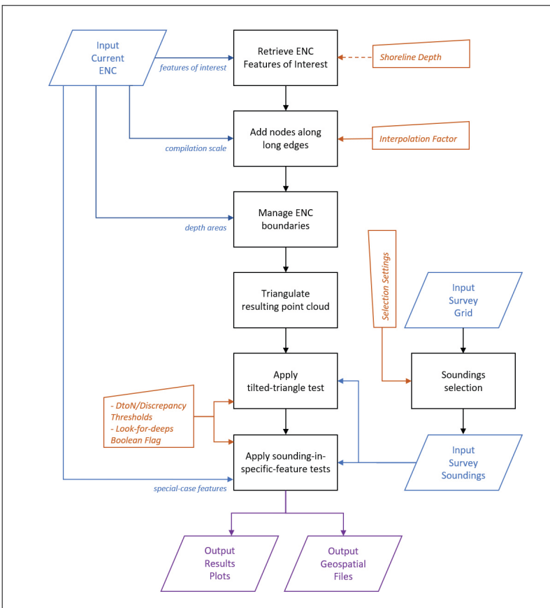
Figure 15-7. Flowchart for CA Tools. The flowchart shows, in black, the main steps of the two combined tools (i.e., Sounding Selection and Chart Comparison). The inputs are represented in blue, the user parameters in orange (with a dashed connector when optional), and the outputs in purple.
