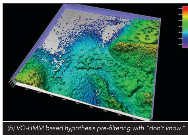
Figure 17-7. Example of depth reconstruction using acoustic-inspired selection rules (a), and the (revised) VQ-HMM approach (b), based on raw (unclassified) LAS files. The noise points in the “standard” selection method (a) are mis-selected reconstructions caused by the density of noise, or lack of actual data, at the estimation points; red points are reconstructions due to surface noise. The VQ-HMM method (b) pre-filters hypotheses and opts to not reconstruct if there are none which resemble the training set’s idea of a sea floor hypothesis.
