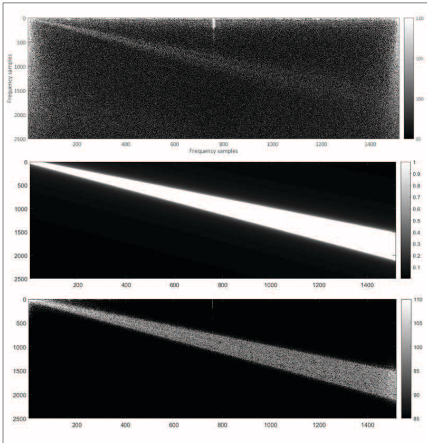
Figure 20-6. Two-dimensional Fourier transform of the Biloxi Dome data (top panel), flat-top filter used to isolate the response of the bubbles (middle panel), and the result of the filtering process (bottom panel).
