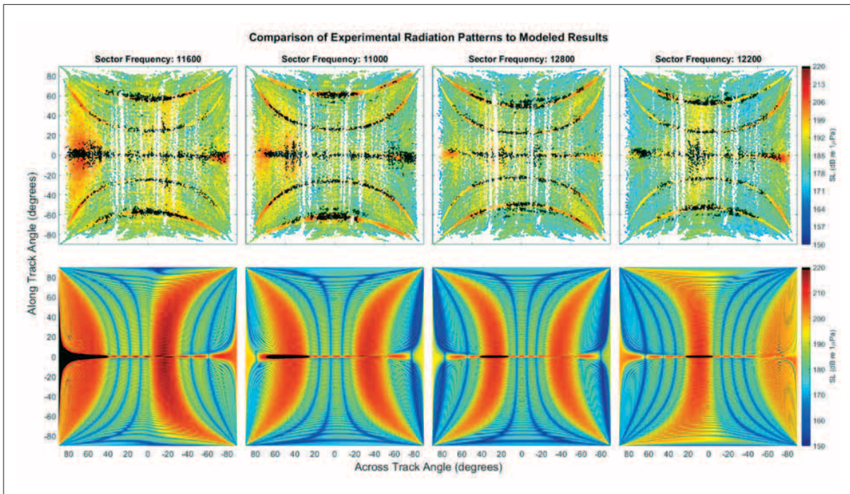
Figure 54-1. Comparison between experimental results and theoretical models of the EM122 radiation patterns of the portside sector of the first swath. The data are plotted in athwartship versus alongship angle. The color corresponds to the equivalent far field source level at 1m. Black within the experimental data corresponds to clipped detections and in the model provides estimates of where clipping was expected.
