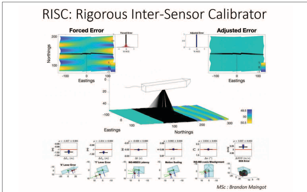
Figure 7-3. Input wobbled seafloor (top-left), the selection of the swath corridor (center), the resulting local and asymptotic estimation of the six integration errors (bottom) and finally the resulting de-wobbled surface (top right).
