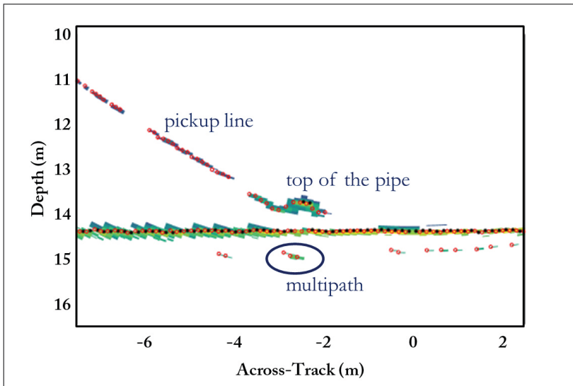
Figure 14-5. A single snapshot showing the result of our multi-detect process including the seafloor the top of the pipe, and the pick-up line used to deploy/recover the pipe.
