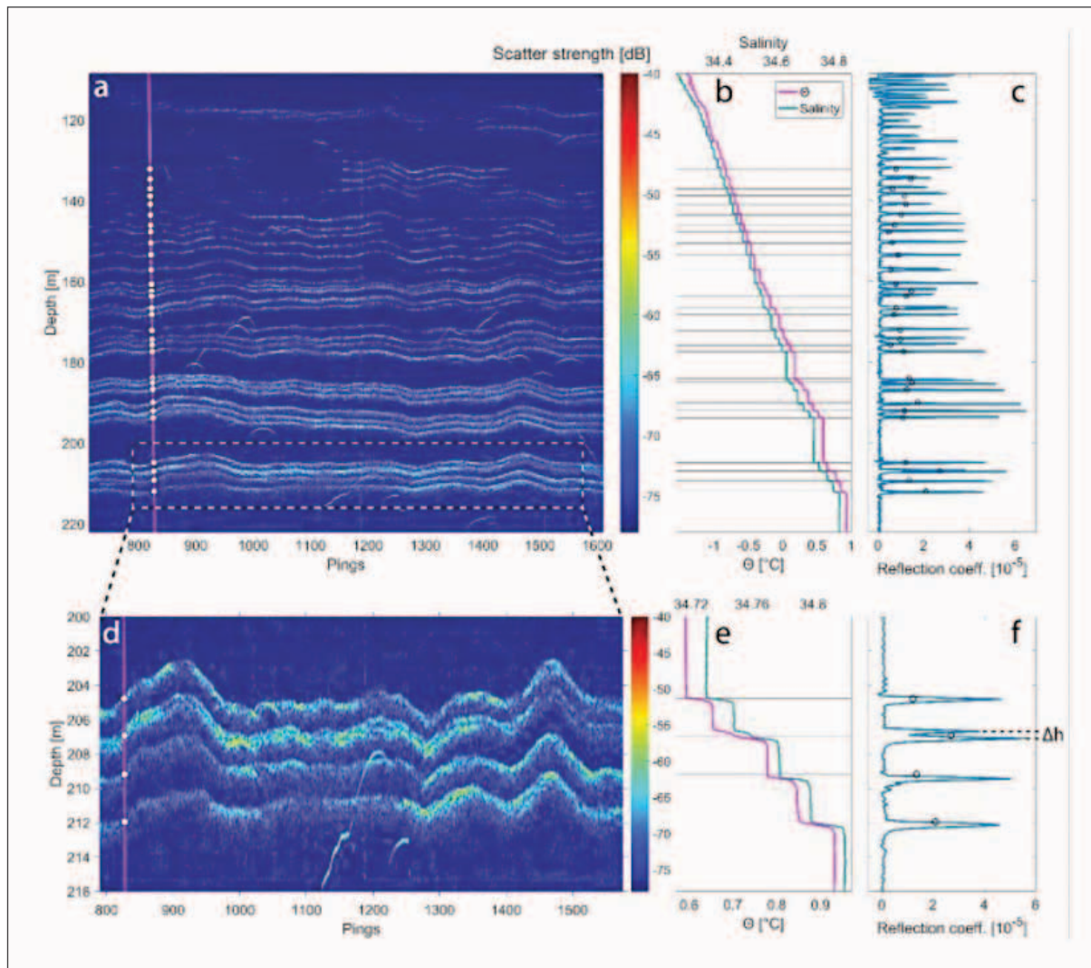
Figure 51-4. Acoustic observations of a thermohaline staircase. a, Processed EK-80 echogram with 8 ms pulse length covering 2.5 hr and a distance of 7 km, with CTD cast (magenta line) and layer depths derived from the echogram scatter strength (white circles). b, CTD potential temperature with reference at the surface ( \Theta ) and salinity profiles with black horizontal lines indicating the depth of the individual layers identified in the echogram (white circles in a). c, reflection coefficient derived from CTD salinity and temperature profiles (blue line) and reflection coefficients estimated from the calibrated target strength in each layer (black circles) at depths derived from the echogram (white circles in a). d-f, same as a-c but over the narrower depth range indicated in the dashed box in a. \Delta h ( = 0.4\text{m} ) in f is the distance between two reflection coefficient peaks, partly visible in d, and represents the minimum spacing visually separable between acoustic horizons (observed vertical resolution). Echoes from fish are seen throughout the data (a,d) as irregular, sometimes hyperbolic, traces.
