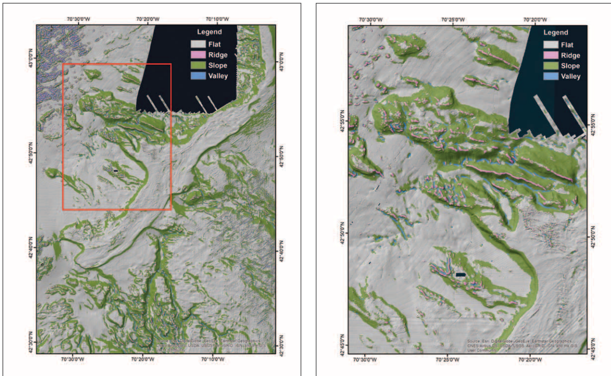
Figure 21-4. Enlargement of the BRESS landform analysis of the bathymetry shown in Figure 21-3 (left panel). The left panel above includes Jeffreys Ledge (running diagonally across figure), large drumline-like features to the northwest (red box) and subglacial drainage channels to the south. The right panel is an enlargement of the area outlined in red. Note the slopes and ridges are clearly defined on the glacial features.
