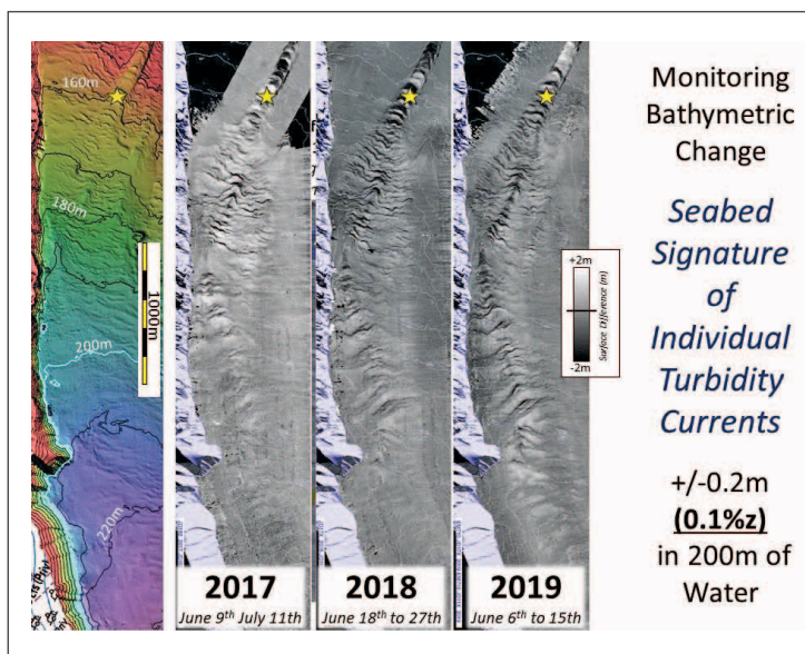
Figure 30-1. Showing the definition of seabed depth changes associated with migrating supercritical bedforms on a submarine fan lobe in ~200m of water. Typical depth changes are at the +/-0.1% of depth scale. These changes are a result of singular turbidity current flows which typically exit the channel mouth (indicated by yellow stars) at ~5m/s (10 knots).
