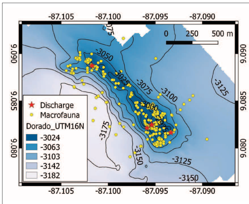
Figure 50-8. Map of Dorado Outcrop showing the distribution of macrofauna and sites of fluid discharge. Yellow circles show macrofauna distribution; Red stars show discharge distribution.
