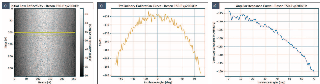
Figure 22-6. Example of the extraction of an angular response curve (pane ‘c’) from the original Reson s7k raw data (pane ‘a’), obtained after application of a preliminary calibration curve (pane ‘b’) and ensemble averaging over 12 pings (yellow area in pane ‘a’).
