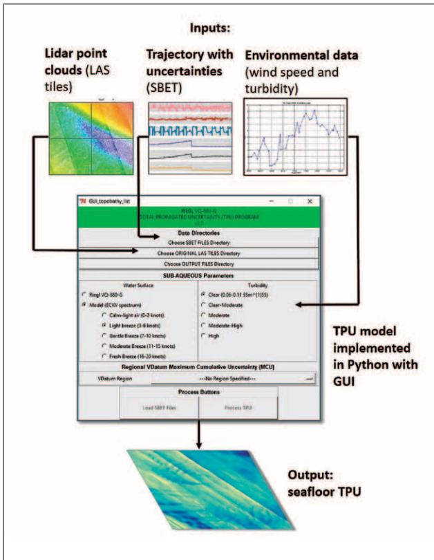
Figure 17-2. Overview of cBLUE software, including inputs and output.
