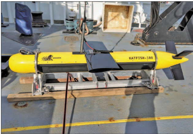
Figure 4-1. The KATFISH system on the deck of the Okeanos Explorer .
