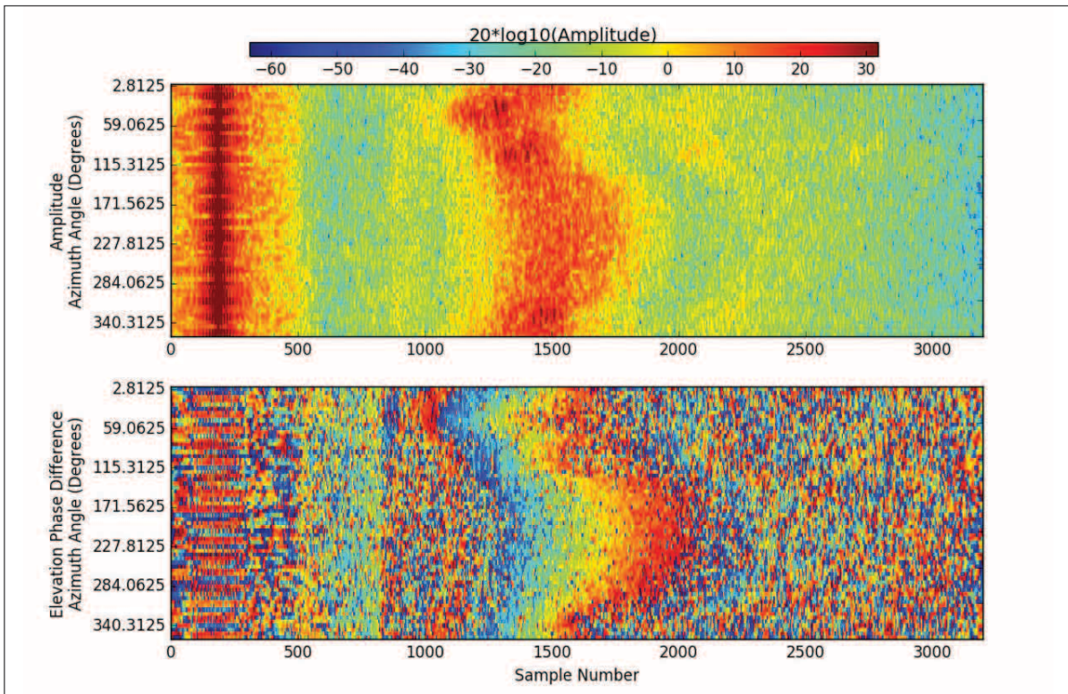
Figure 3-2. Raw amplitude (top) and phase (bottom) data collected with an SU90. The seafloor is apparent with high amplitude and quasi-linear phase between samples 1000-2000.
