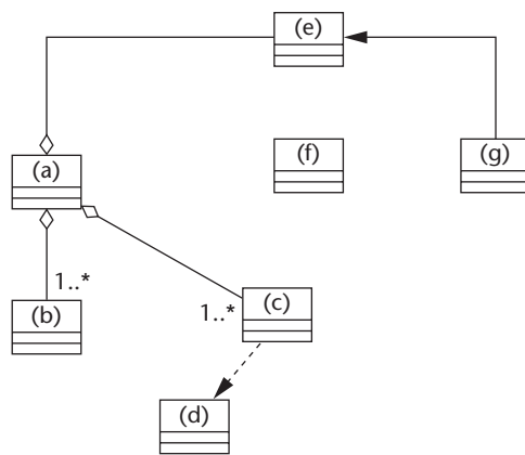
18 The UML representation equivalent to the Figure 17's geon representation.
