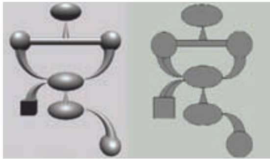
5 A geon diagram and an equivalent 2D-silhouette diagram.
